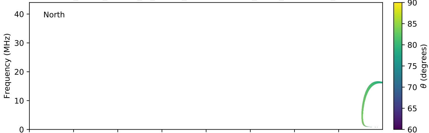
expres_earth_jupiter_io_jrm09_lossc-wid1deg_3kev_20150509_v01.cdf
