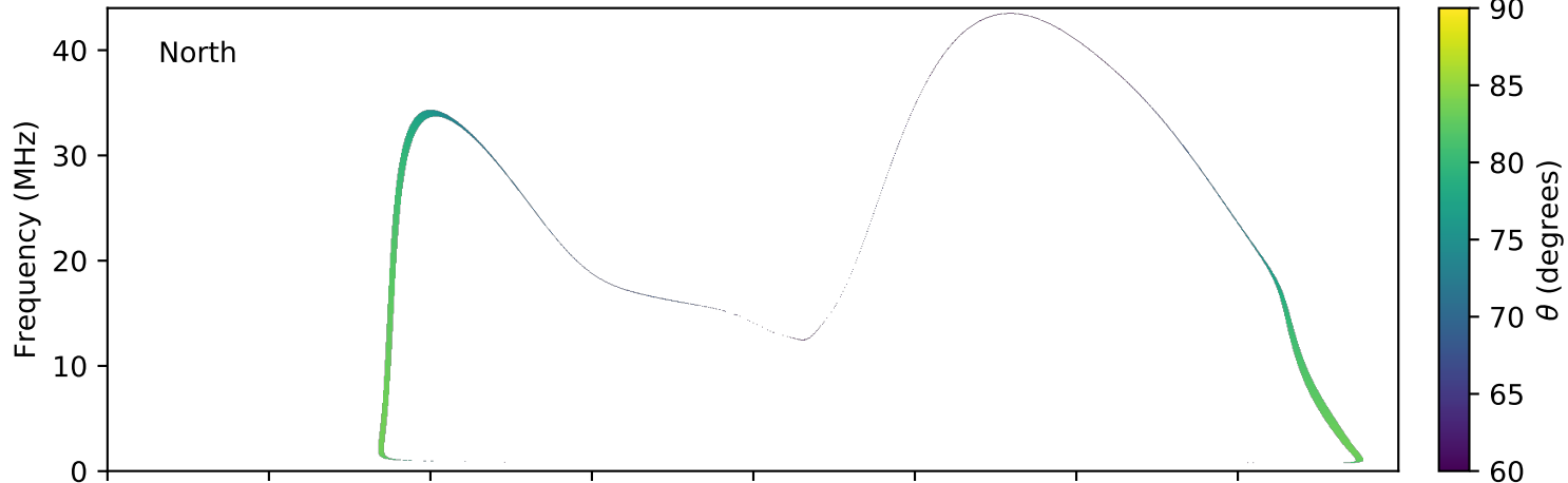
expres_earth_jupiter_io_jrm09_lossc-wid1deg_3kev_20150508_v01.cdf
