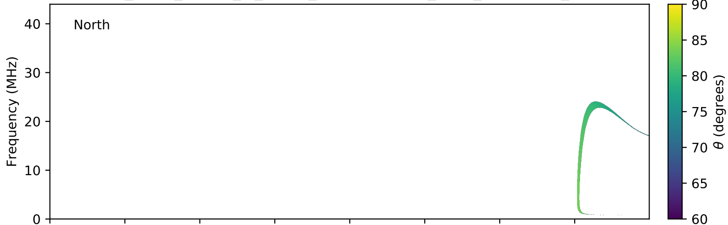
expres_earth_jupiter_io_jrm09_lossc-wid1deg_3kev_20150502_v01.cdf
