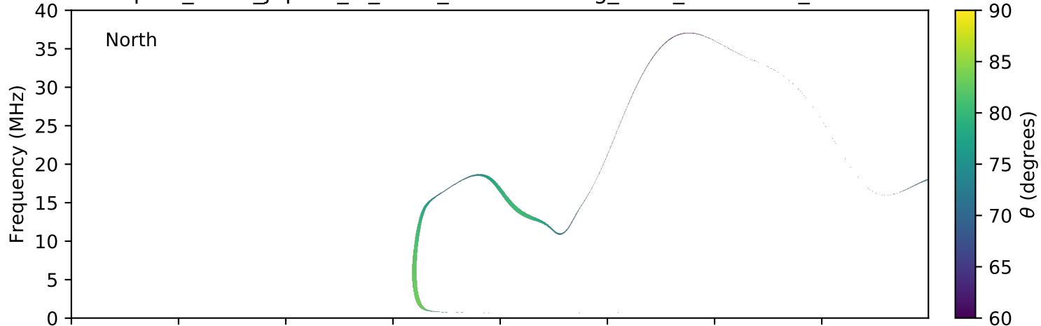
expres_earth_jupiter_io_isaac_lossc-wid1deg_3kev_20150529_v01.cdf
