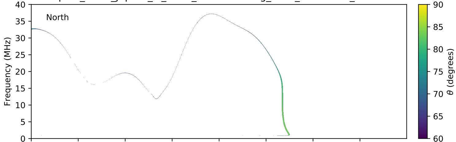
expres_earth_jupiter_io_isaac_lossc-wid1deg_3kev_20150526_v01.cdf
