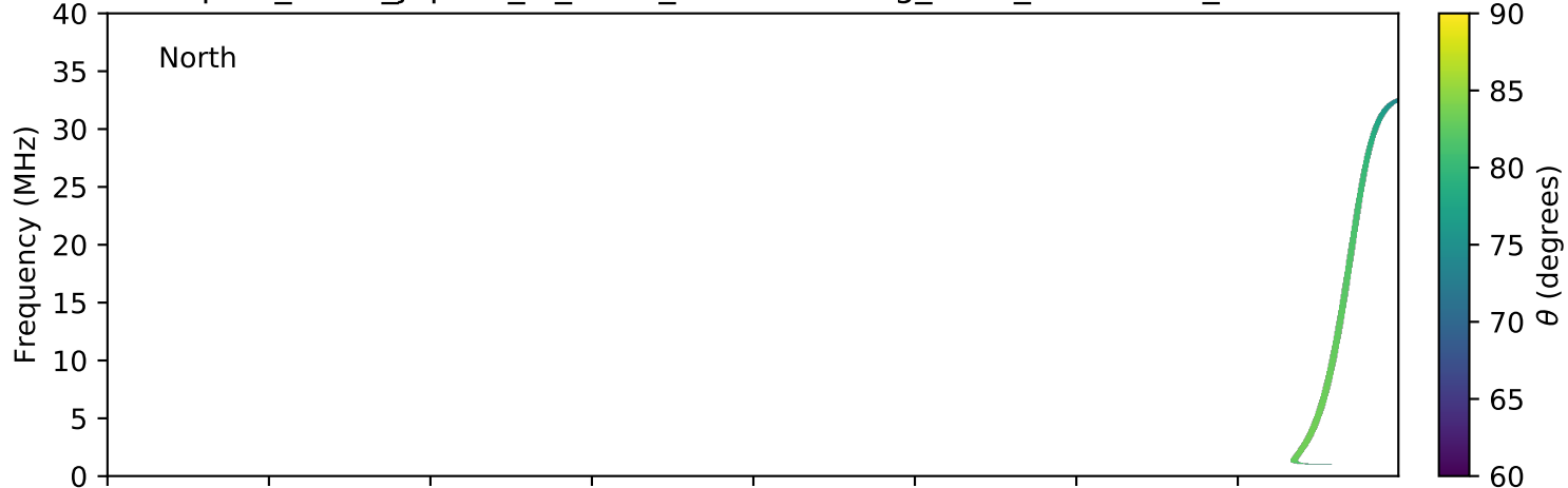
expres_earth_jupiter_io_isaac_lossc-wid1deg_3kev_20150525_v01.cdf
