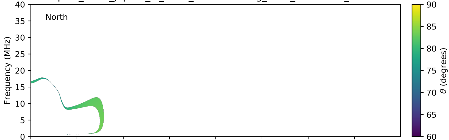
expres_earth_jupiter_io_isaac_lossc-wid1deg_3kev_20150523_v01.cdf
