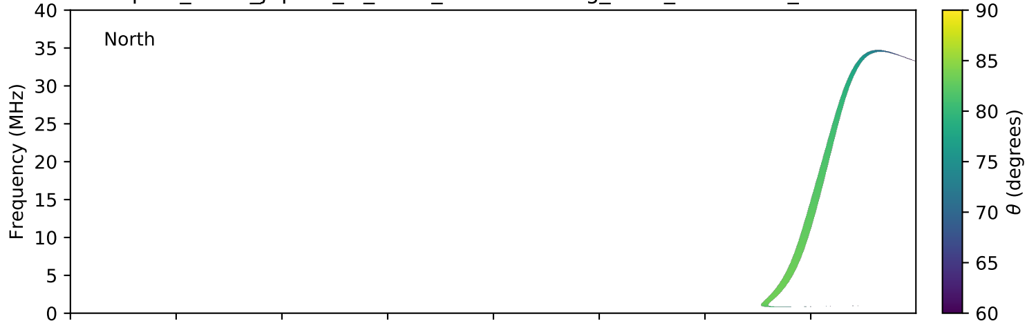
expres_earth_jupiter_io_isaac_lossc-wid1deg_3kev_20150518_v01.cdf
