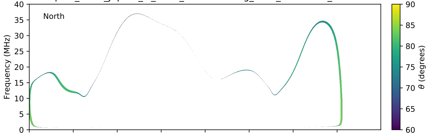
expres_earth_jupiter_io_isaac_lossc-wid1deg_3kev_20150517_v01.cdf
