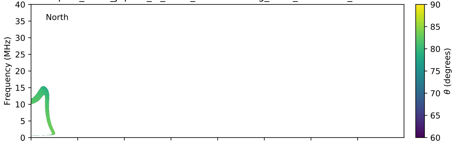
expres_earth_jupiter_io_isaac_lossc-wid1deg_3kev_20150516_v01.cdf
