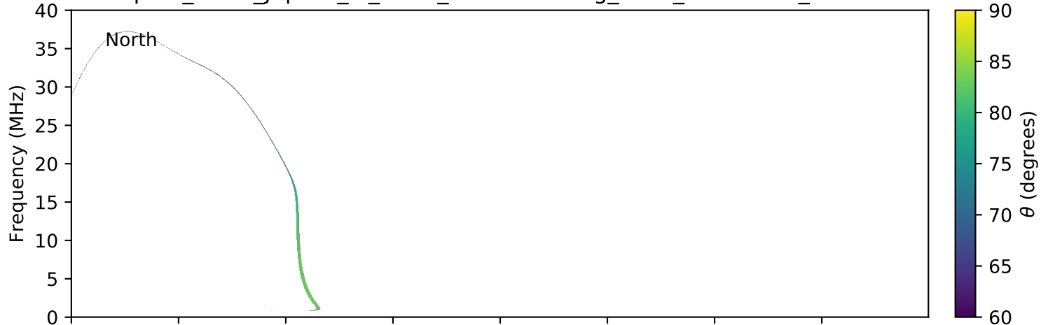
expres_earth_jupiter_io_isaac_lossc-wid1deg_3kev_20150514_v01.cdf
