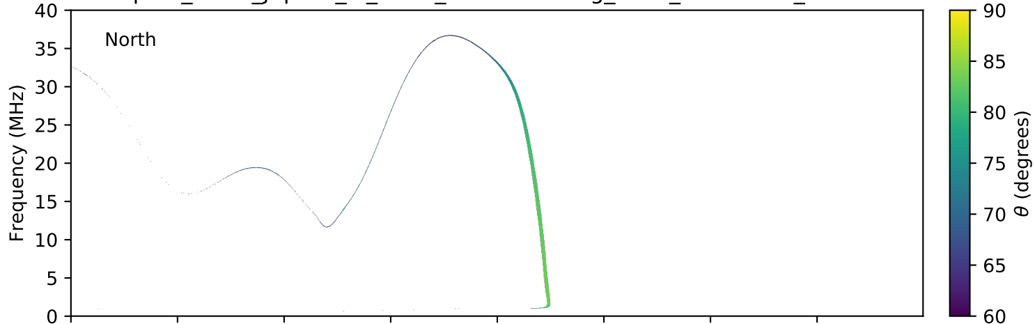
expres_earth_jupiter_io_isaac_lossc-wid1deg_3kev_20150512_v01.cdf
