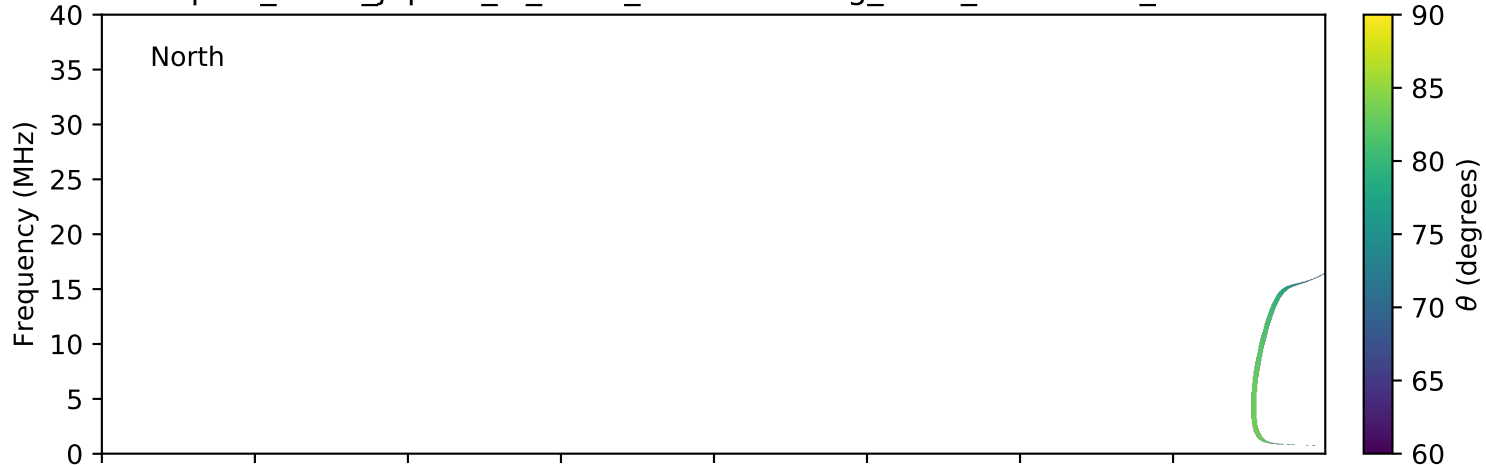
expres_earth_jupiter_io_isaac_lossc-wid1deg_3kev_20150509_v01.cdf
