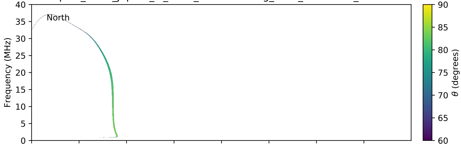
expres_earth_jupiter_io_isaac_lossc-wid1deg_3kev_20150507_v01.cdf
