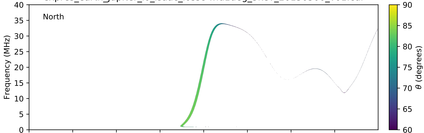
expres_earth_jupiter_io_isaac_lossc-wid1deg_3kev_20150506_v01.cdf
