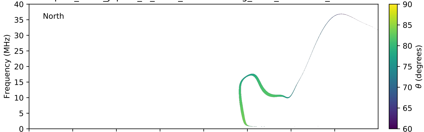
expres_earth_jupiter_io_isaac_lossc-wid1deg_3kev_20150504_v01.cdf
