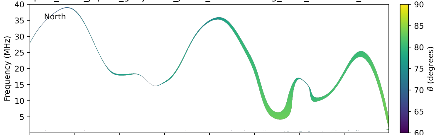
expres_earth_jupiter_ganymede_jrm33_lossc-wid1deg_3kev_20150507_v11.cdf
