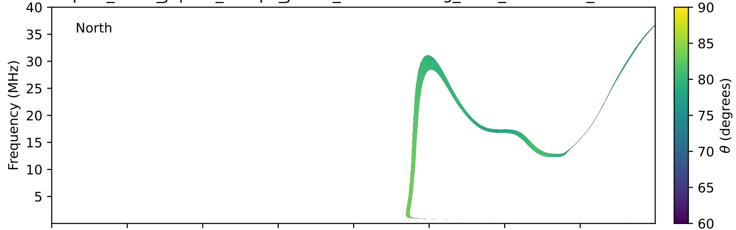
expres_earth_jupiter_europa_jrm33_lossc-wid1deg_3kev_20150513_v11.cdf
