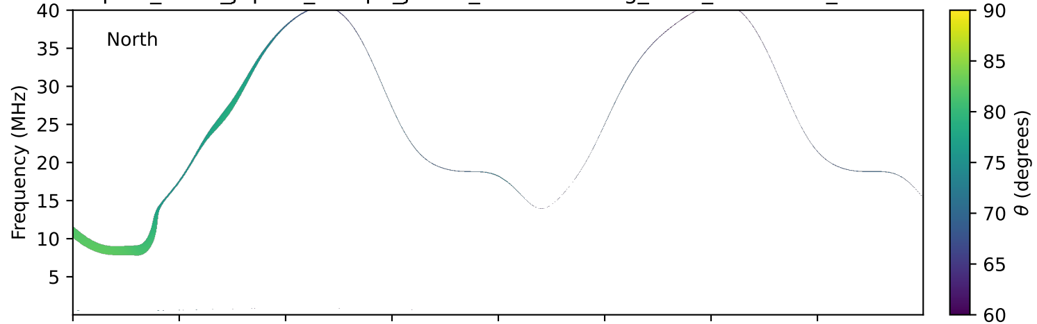
expres_earth_jupiter_europa_jrm33_lossc-wid1deg_3kev_20150503_v11.cdf
