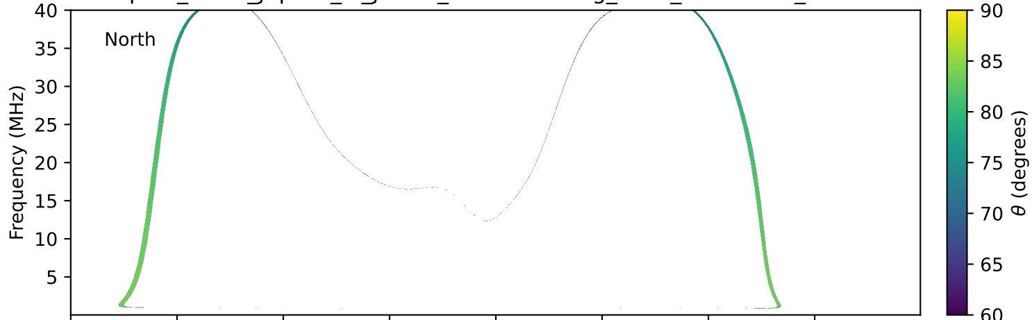
expres_earth_jupiter_io_jrm33_lossc-wid1deg_3kev_20150424_v11.cdf
