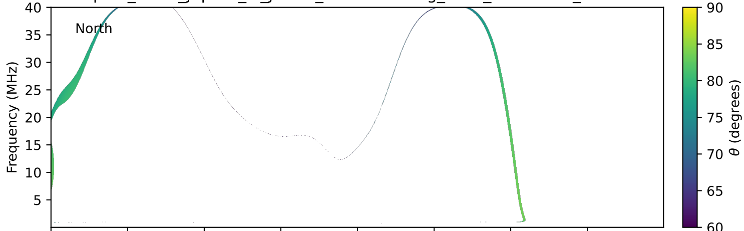
expres_earth_jupiter_io_jrm33_lossc-wid1deg_3kev_20150417_v11.cdf
