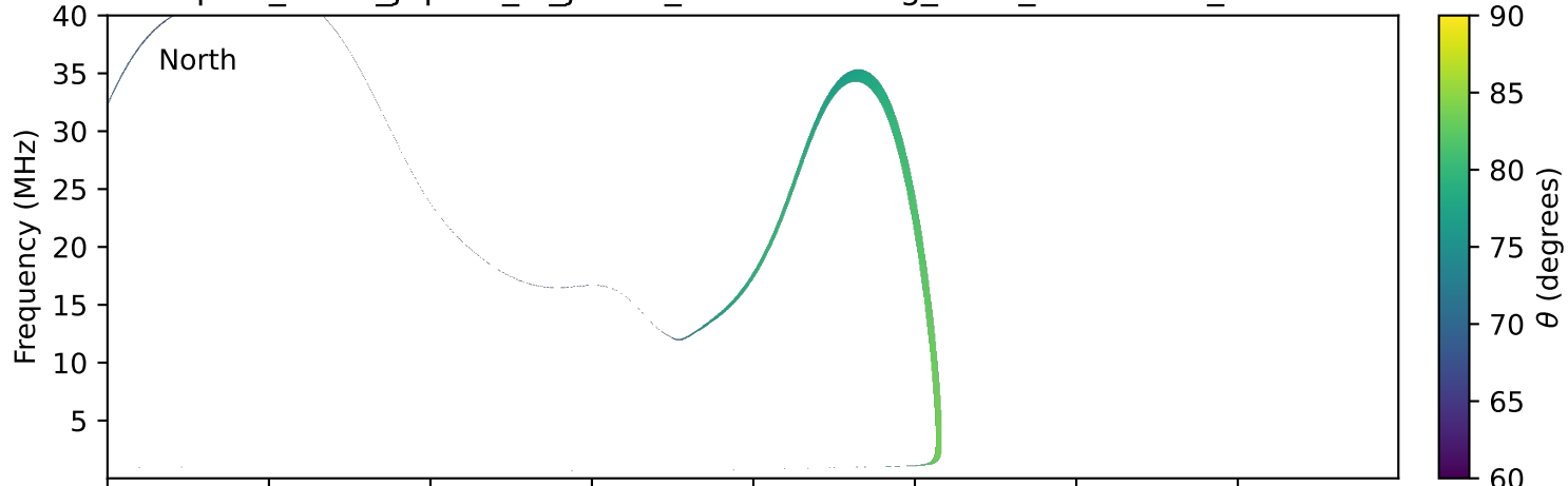
expres_earth_jupiter_io_jrm33_lossc-wid1deg_3kev_20150403_v11.cdf
