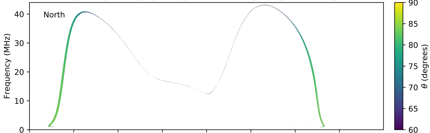
expres_earth_jupiter_io_jrm09_lossc-wid1deg_3kev_20150424_v01.cdf
