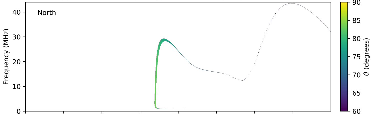
expres_earth_jupiter_io_jrm09_lossc-wid1deg_3kev_20150413_v01.cdf
