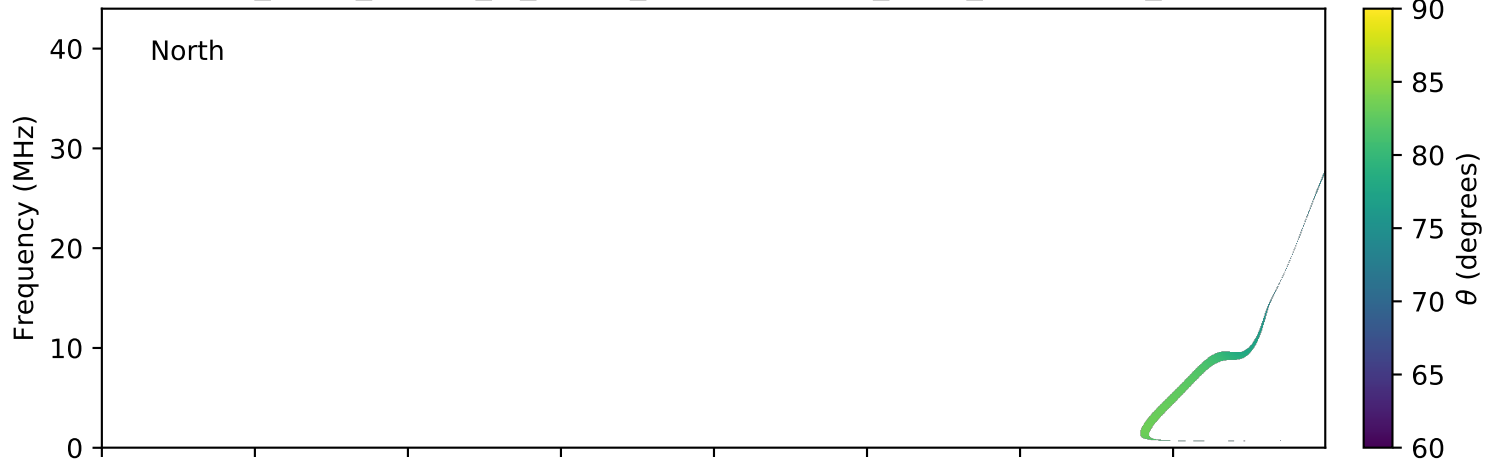
expres_earth_jupiter_io_jrm09_lossc-wid1deg_3kev_20150409_v01.cdf
