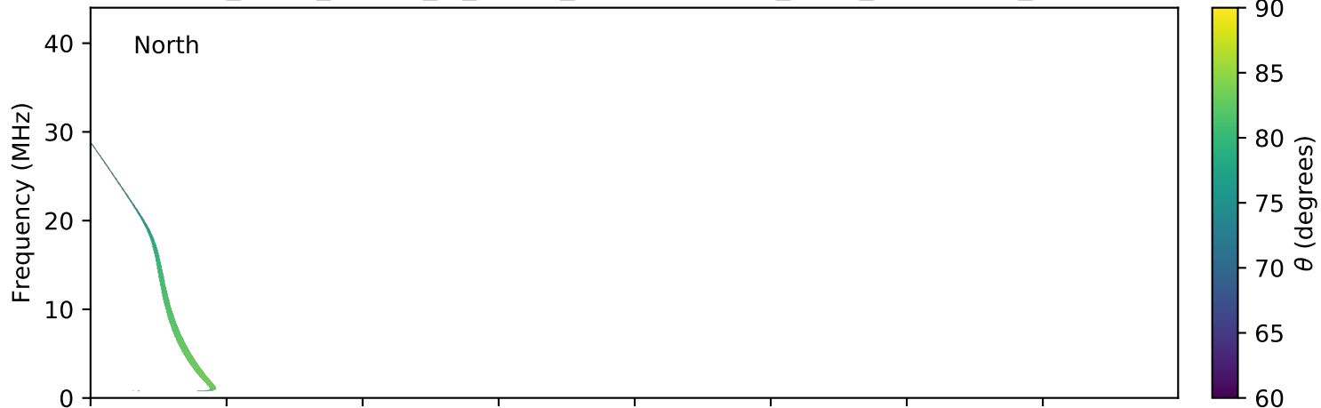
expres_earth_jupiter_io_jrm09_lossc-wid1deg_3kev_20150407_v01.cdf
