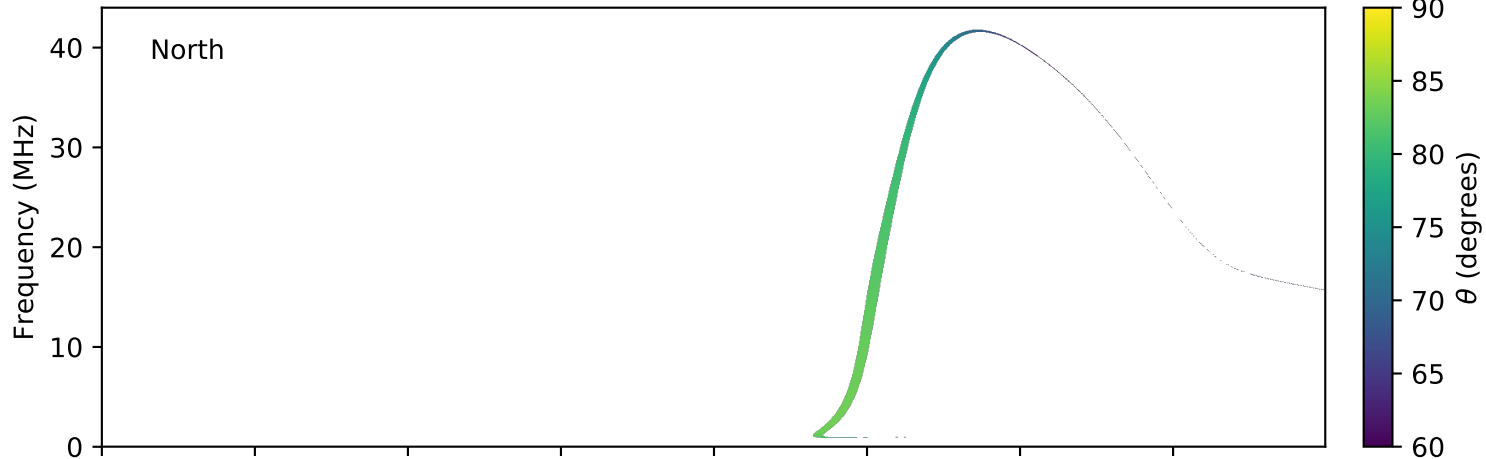
expres_earth_jupiter_io_jrm09_lossc-wid1deg_3kev_20150404_v01.cdf
