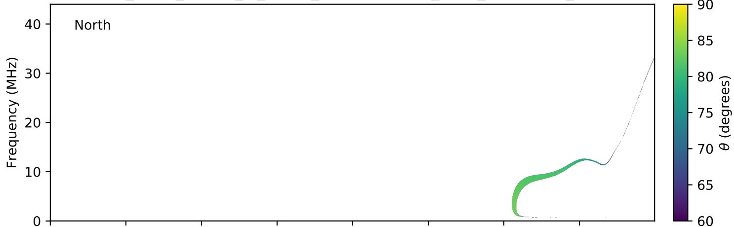
expres_earth_jupiter_io_jrm09_lossc-wid1deg_3kev_20150402_v01.cdf
