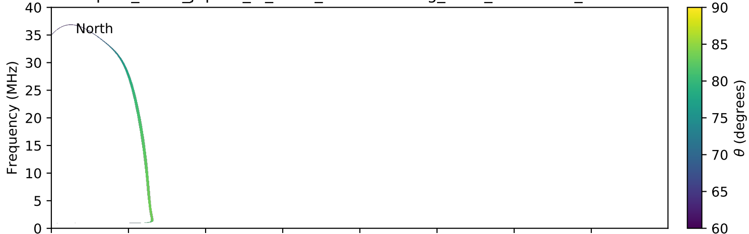
expres_earth_jupiter_io_isaac_lossc-wid1deg_3kev_20150430_v01.cdf
