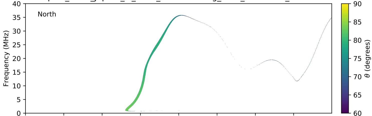
expres_earth_jupiter_io_isaac_lossc-wid1deg_3kev_20150429_v01.cdf
