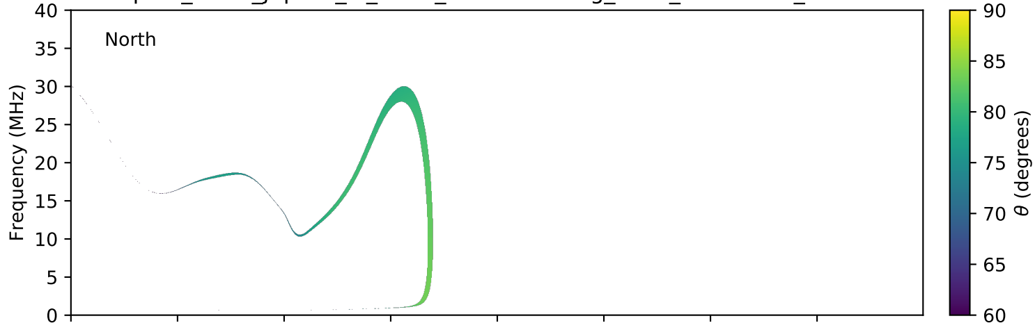
expres_earth_jupiter_io_isaac_lossc-wid1deg_3kev_20150428_v01.cdf
