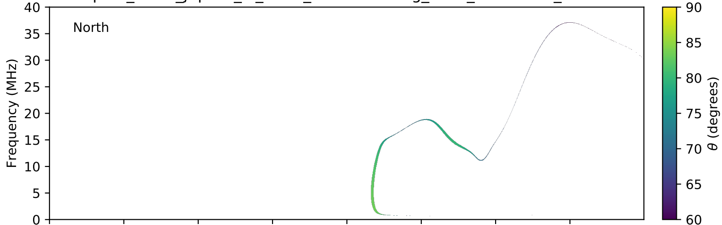
expres_earth_jupiter_io_isaac_lossc-wid1deg_3kev_20150427_v01.cdf
