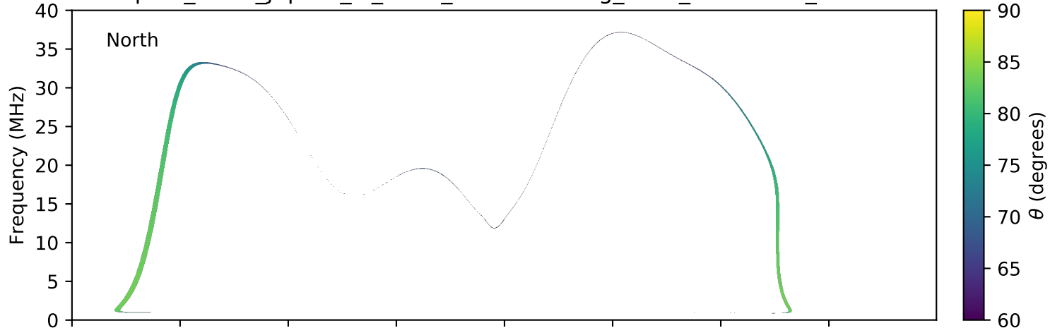
expres_earth_jupiter_io_isaac_lossc-wid1deg_3kev_20150424_v01.cdf
