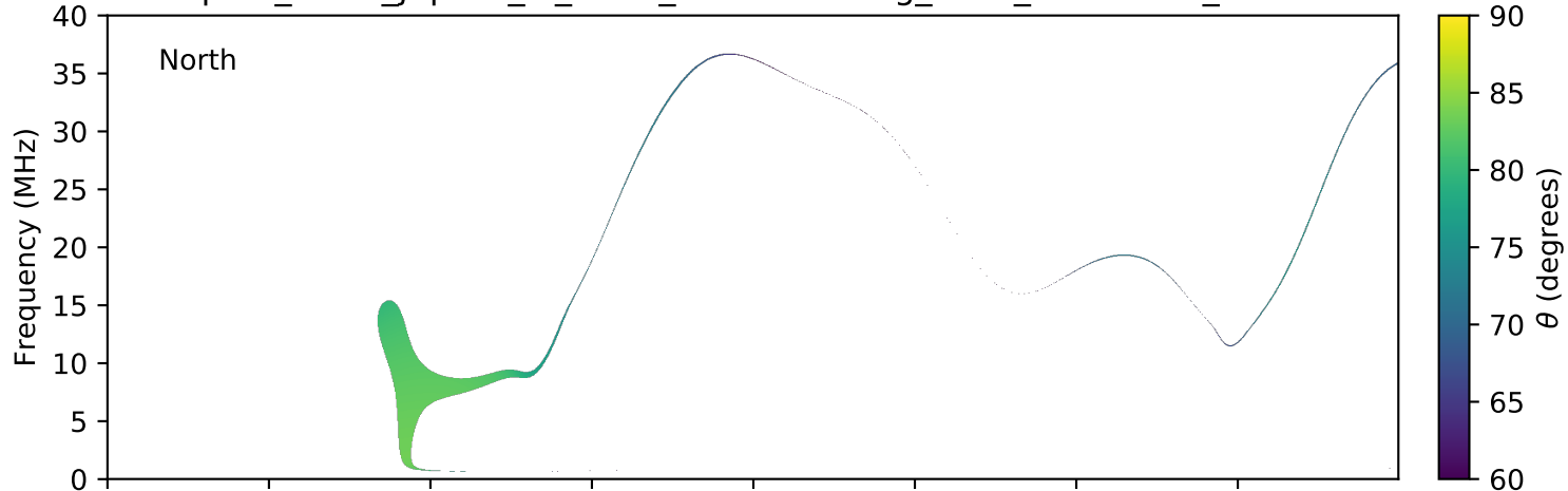
expres_earth_jupiter_io_isaac_lossc-wid1deg_3kev_20150422_v01.cdf
