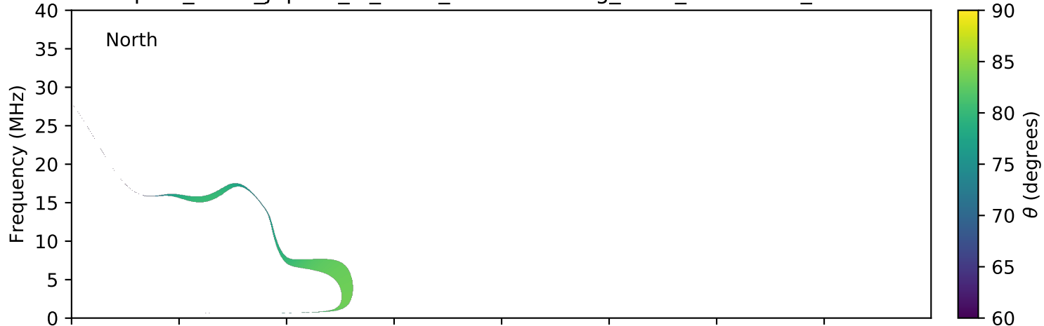
expres_earth_jupiter_io_isaac_lossc-wid1deg_3kev_20150421_v01.cdf
