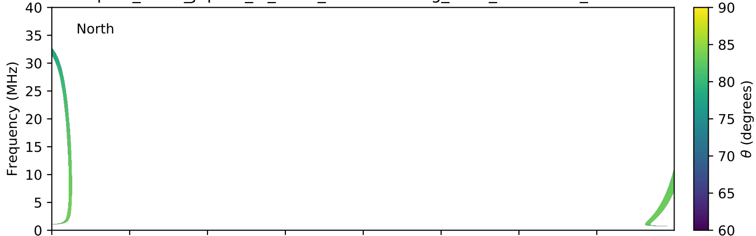
expres_earth_jupiter_io_isaac_lossc-wid1deg_3kev_20150416_v01.cdf
