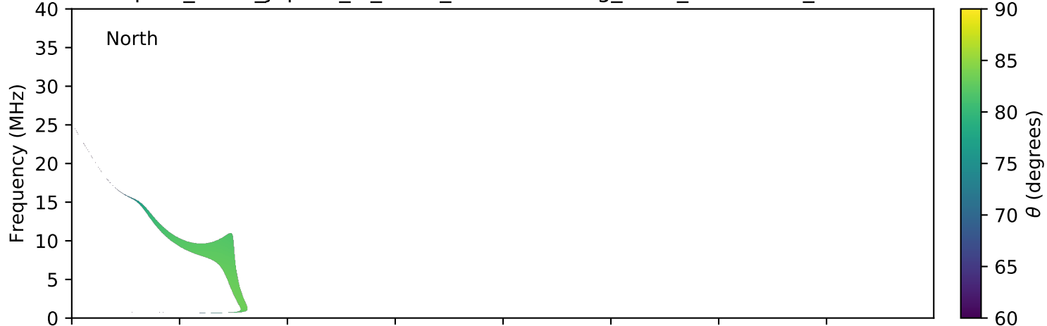
expres_earth_jupiter_io_isaac_lossc-wid1deg_3kev_20150414_v01.cdf
