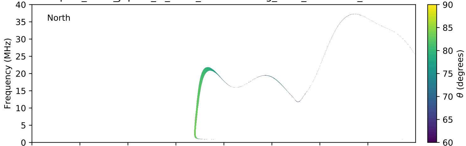
expres_earth_jupiter_io_isaac_lossc-wid1deg_3kev_20150413_v01.cdf
