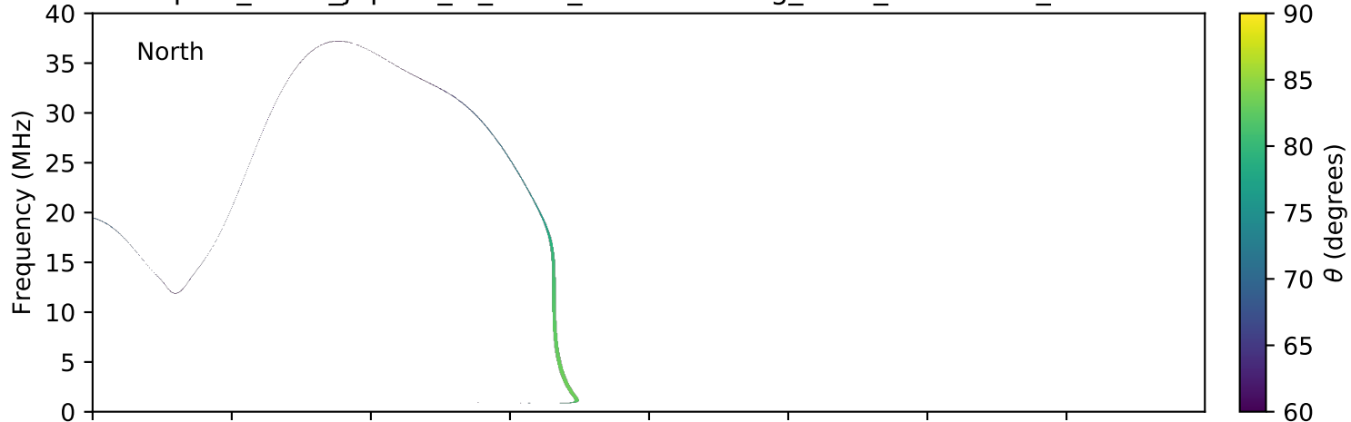
expres_earth_jupiter_io_isaac_lossc-wid1deg_3kev_20150412_v01.cdf
