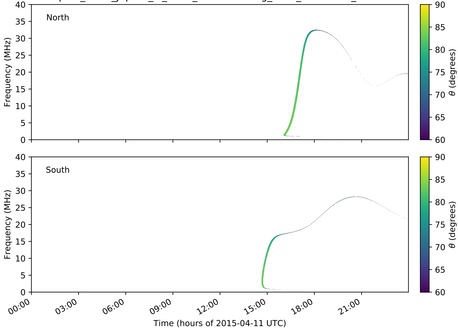
expres_earth_jupiter_io_isaac_lossc-wid1deg_3kev_20150411_v01.cdf
