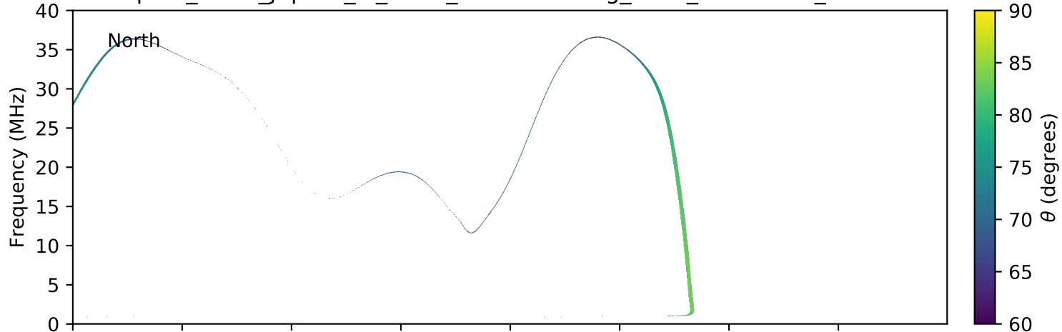
expres_earth_jupiter_io_isaac_lossc-wid1deg_3kev_20150410_v01.cdf
