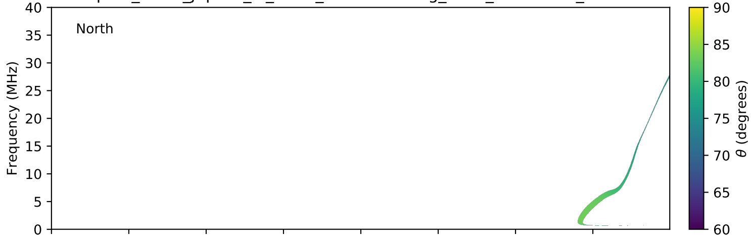
expres_earth_jupiter_io_isaac_lossc-wid1deg_3kev_20150409_v01.cdf
