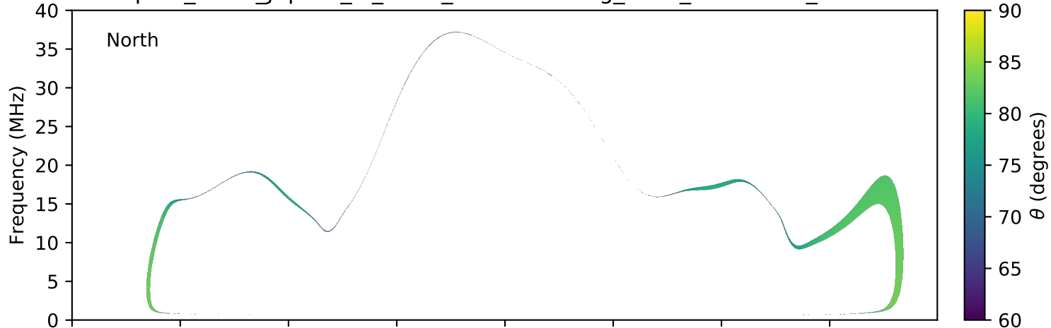
expres_earth_jupiter_io_isaac_lossc-wid1deg_3kev_20150408_v01.cdf
