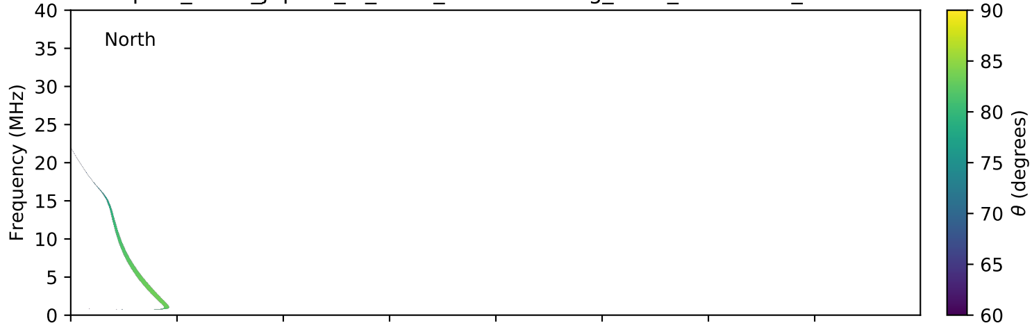
expres_earth_jupiter_io_isaac_lossc-wid1deg_3kev_20150407_v01.cdf
