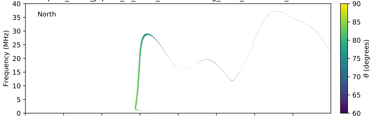
expres_earth_jupiter_io_isaac_lossc-wid1deg_3kev_20150406_v01.cdf
