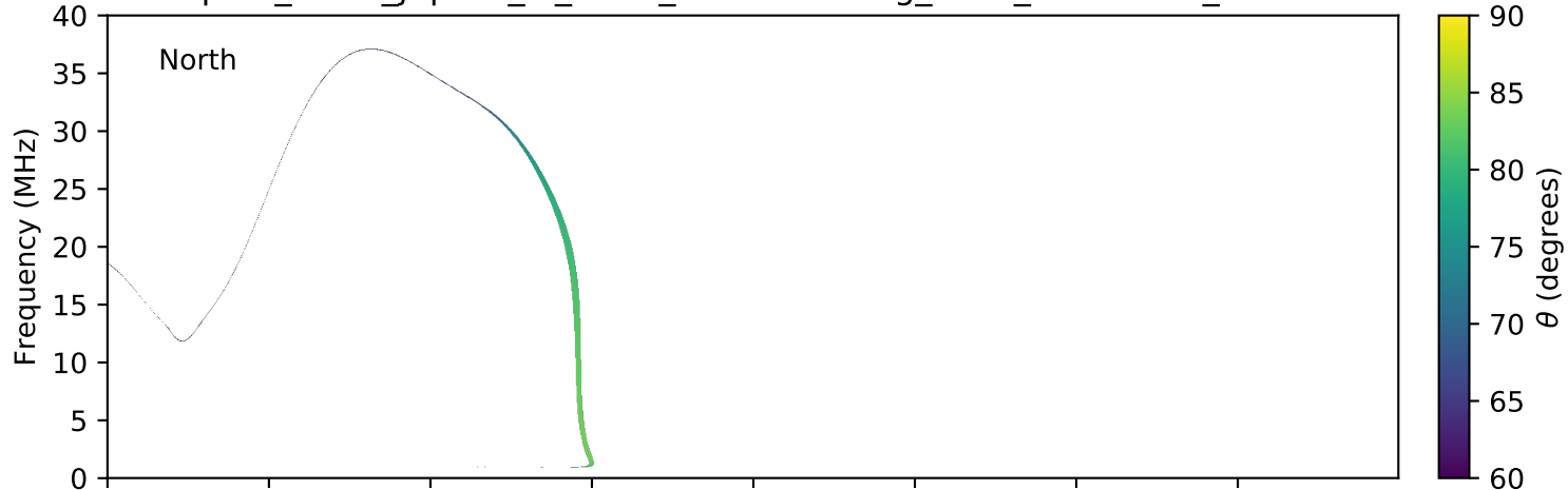
expres_earth_jupiter_io_isaac_lossc-wid1deg_3kev_20150405_v01.cdf
