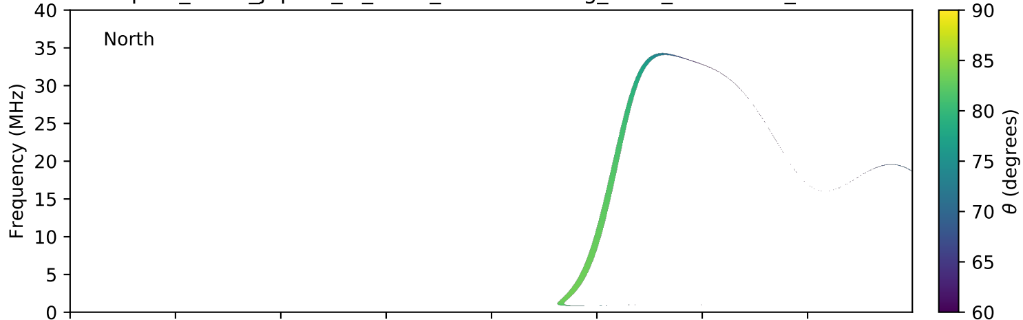
expres_earth_jupiter_io_isaac_lossc-wid1deg_3kev_20150404_v01.cdf
