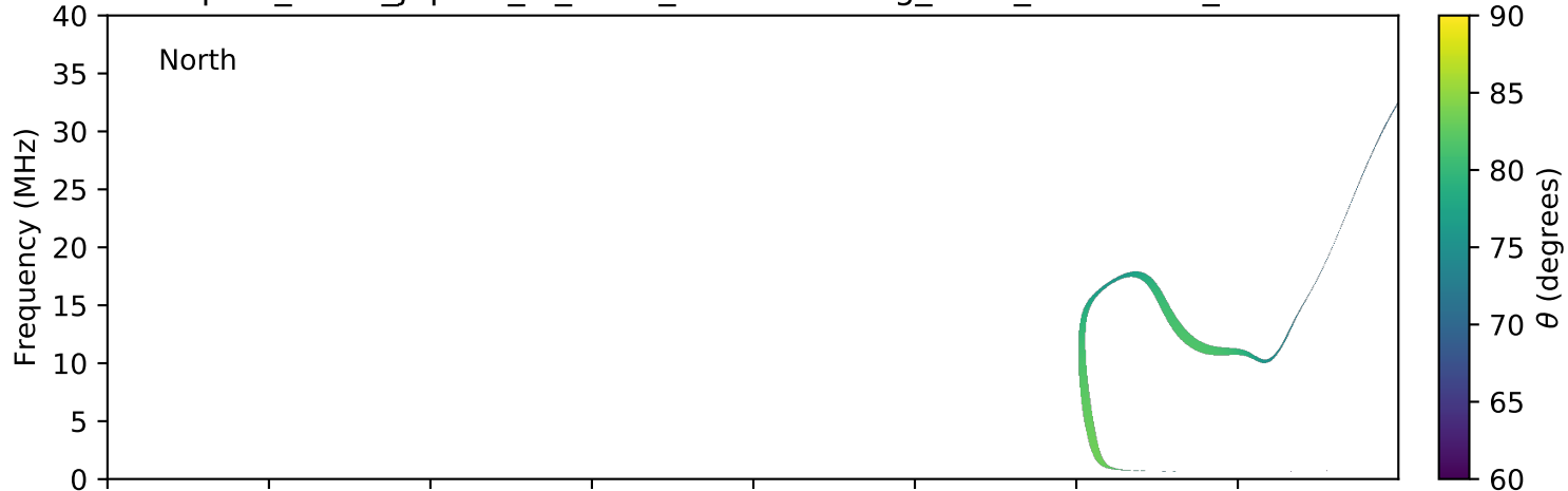
expres_earth_jupiter_io_isaac_lossc-wid1deg_3kev_20150402_v01.cdf
