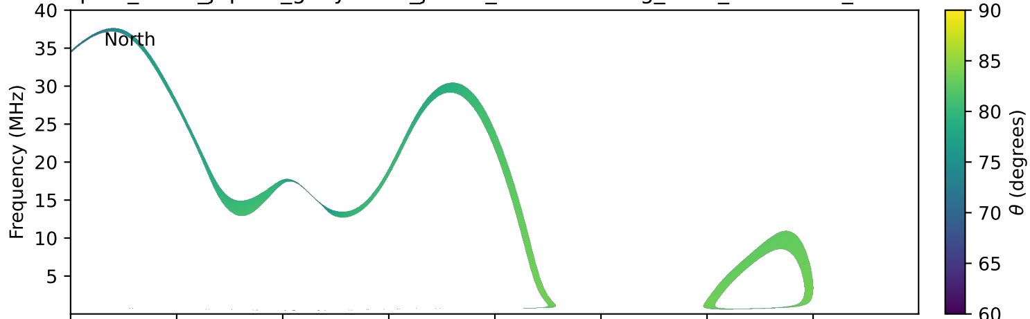
expres_earth_jupiter_ganymede_jrm33_lossc-wid1deg_3kev_20150423_v11.cdf
