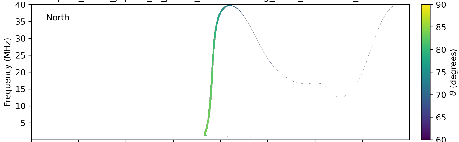
expres_earth_jupiter_io_jrm33_lossc-wid1deg_3kev_20150226_v11.cdf
